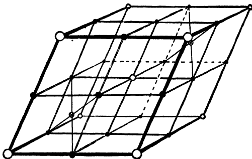
FIG. 2.—The structure calcite would have had if it had crystallized according to type (4) (see text). \odot represents Ca (or C); \circ represents C (or Ca); \bullet represents O.
